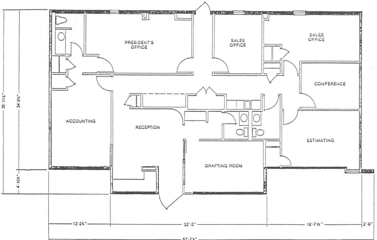
Front Building
